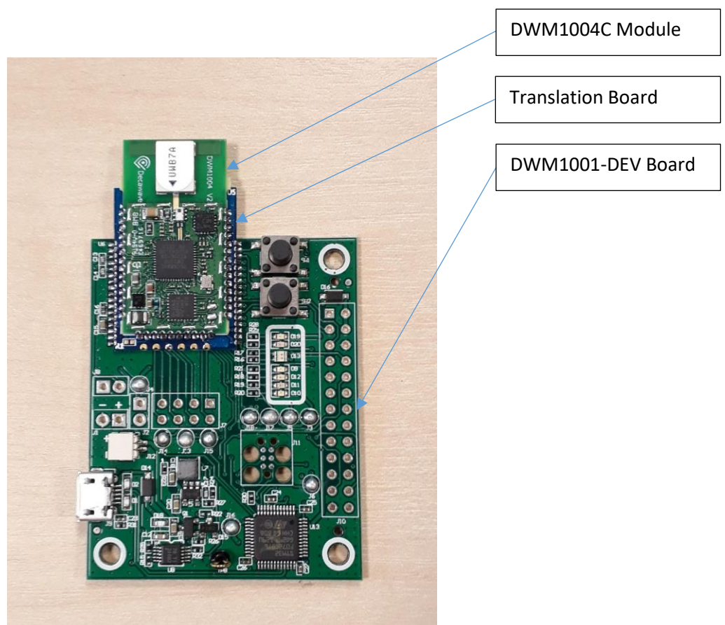
Figure 1 DWM1004C module
